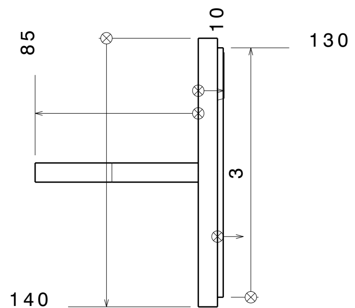
Front view Scale: 1:2
